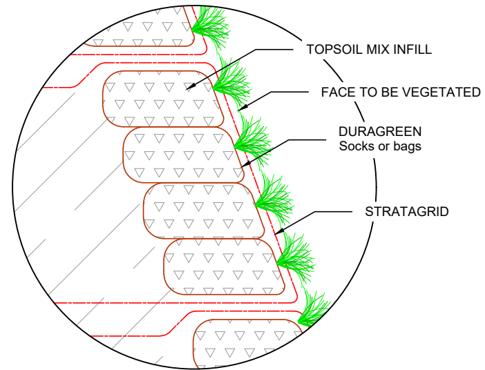
DETAIL A: DURAGREEN FACING SYSTEM
