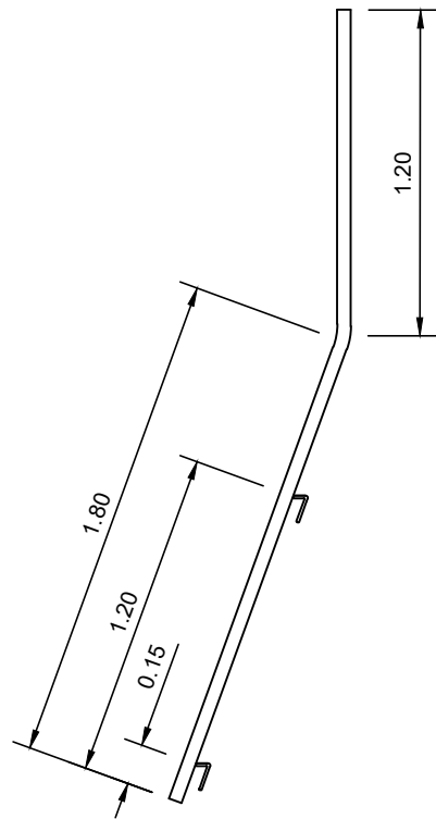
SAFETY RAIL UPRIGHT
